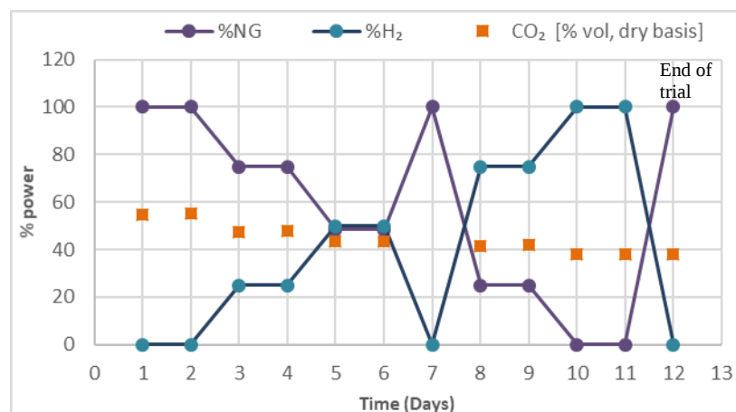
Figure 1. Evolution of Hydrogen and Natural Gas Power Consumption vs. Volumetric CO 2 Percentage
